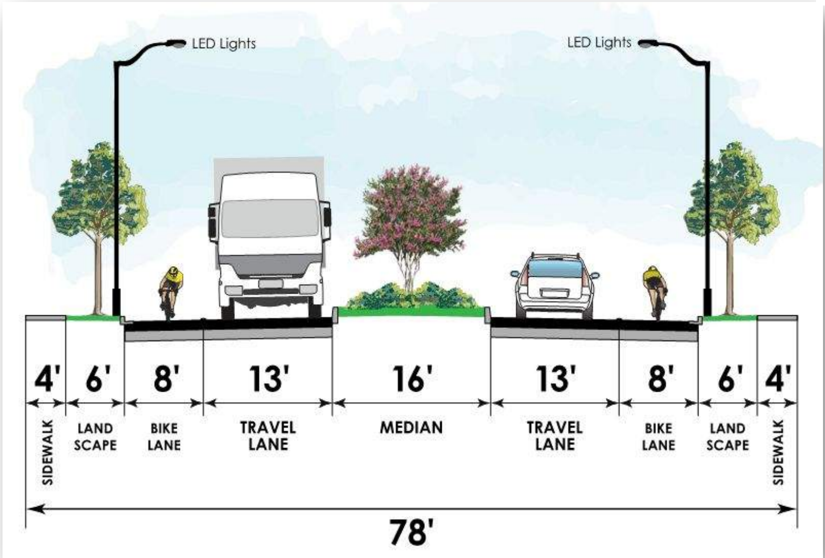
Whitesell Street Cross Section
