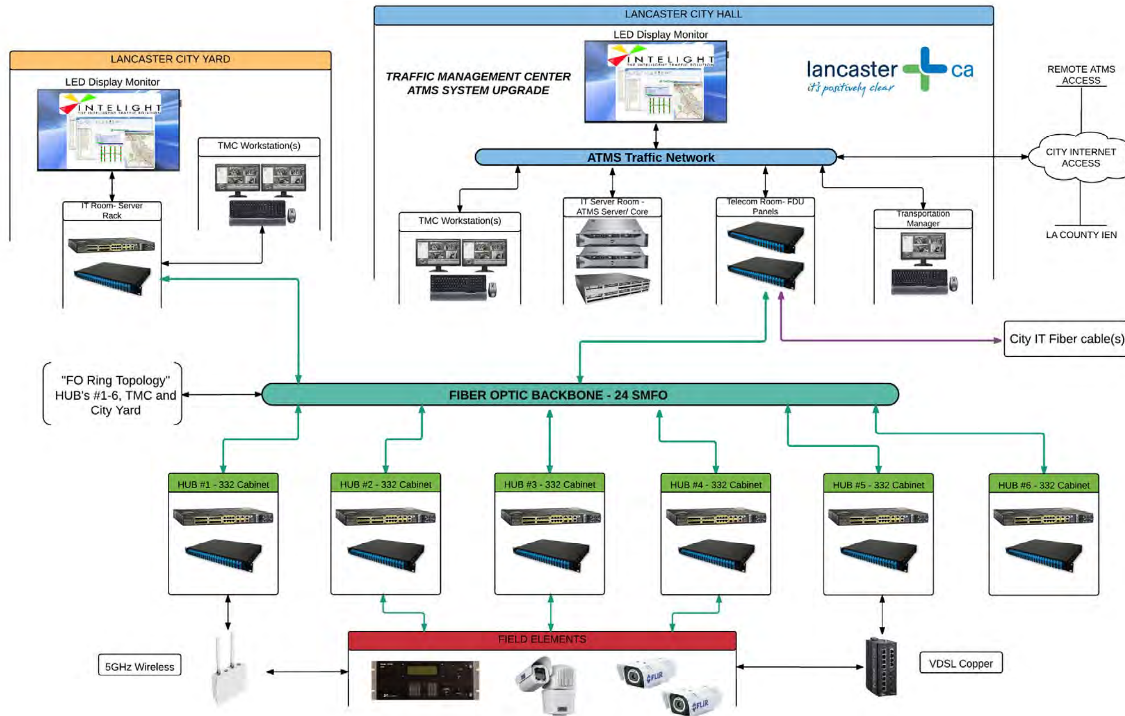
Figure 4.6. ATMS Communications System Architecture and ITS Elements
