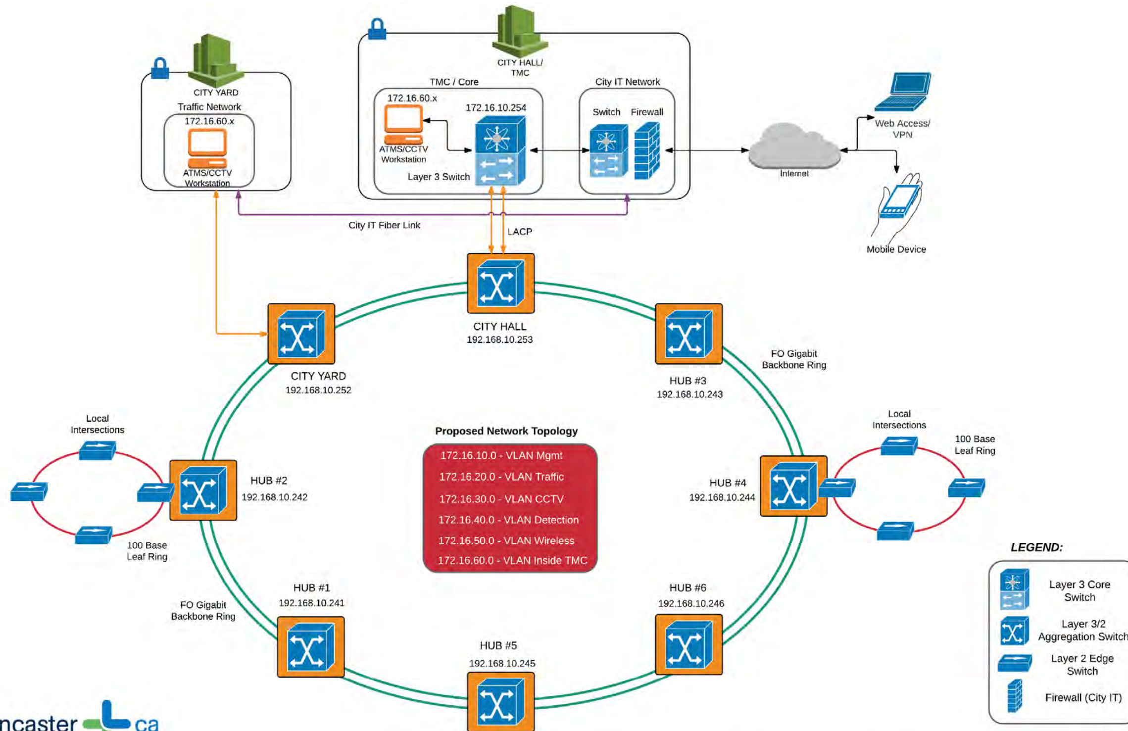
Figure 4.5. Communications Backbone System Architecture
